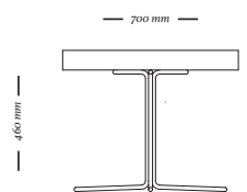
9015 700x700x460mm
